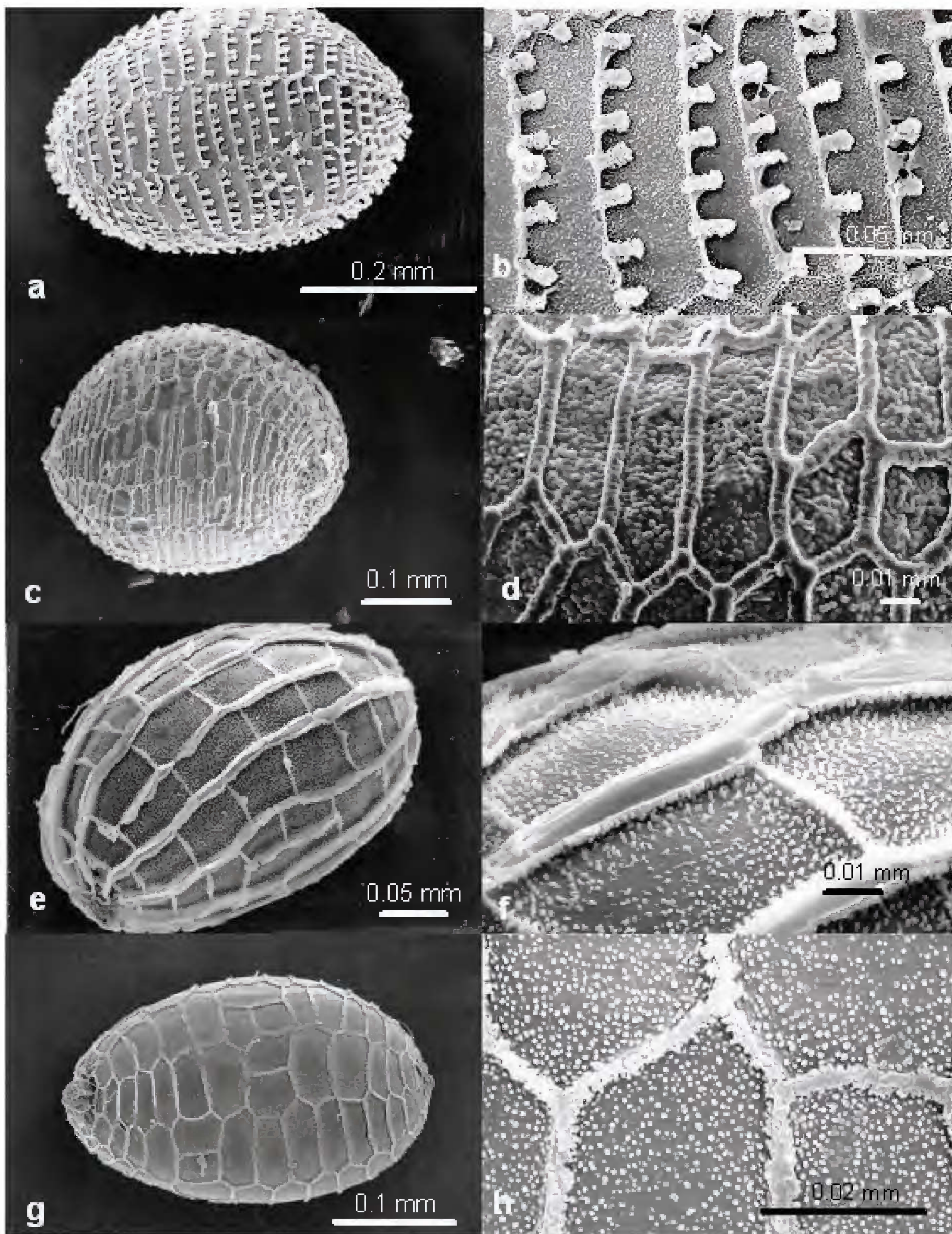
Fig. 7. Seed and seed surface: Eriocaulon odontospermum a, b ; E. patericola c, d ; E. pusillum e, f ; E. pygmaeum g, h . Material used: a-b from Blake 9546 ; c-d from Menkhorst 302 ; e-f from Latz 6305 ; g-h from Banks & Solander BM000900916 .
